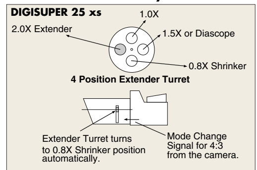
The diagram shows how Canon's exclusive Crossover Technology uses a 0.8X "Shrinker" to restore the loss of diameter and return the 4:3 image of a Switchable Camera to the same as a Standard Camera.
